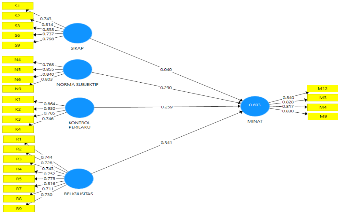
Gambar 1. Output Pengukuran Outer Model
