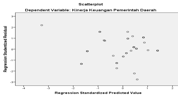
Gambar 2. Hasil Uji Scatterplot
