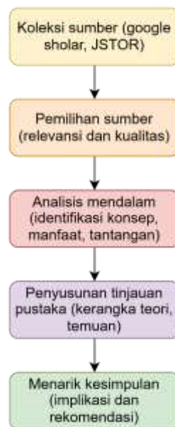
Gambar 1 Alur Penelitian
