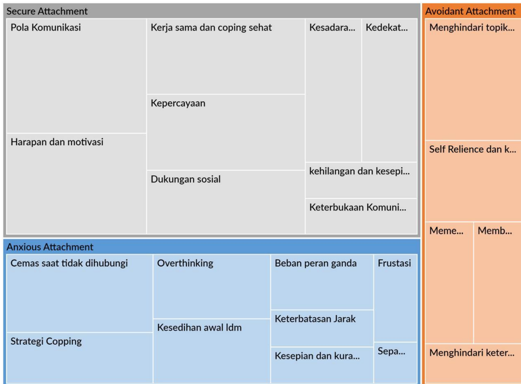
Gambar 7 Hierarchy Chart
